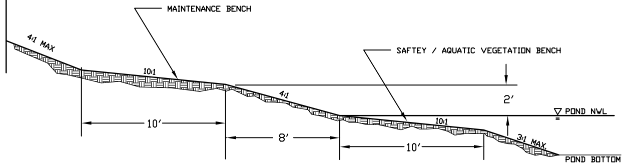
TYPICAL BENCH DETAIL
