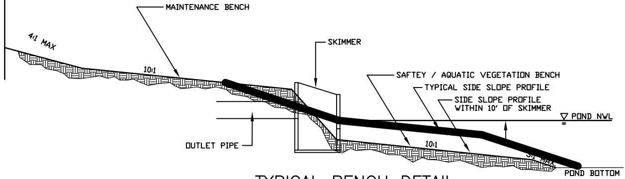
TYPICAL BENCH DETAIL WITHIN 10' OF SKIMMER OUTLET
