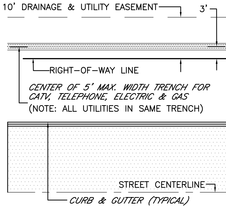
TYPICAL PRIVATE UTILITY PLACEMENT
