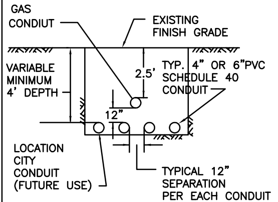
TRENCH CROSS SECTION AT CONDUIT CROSSING
