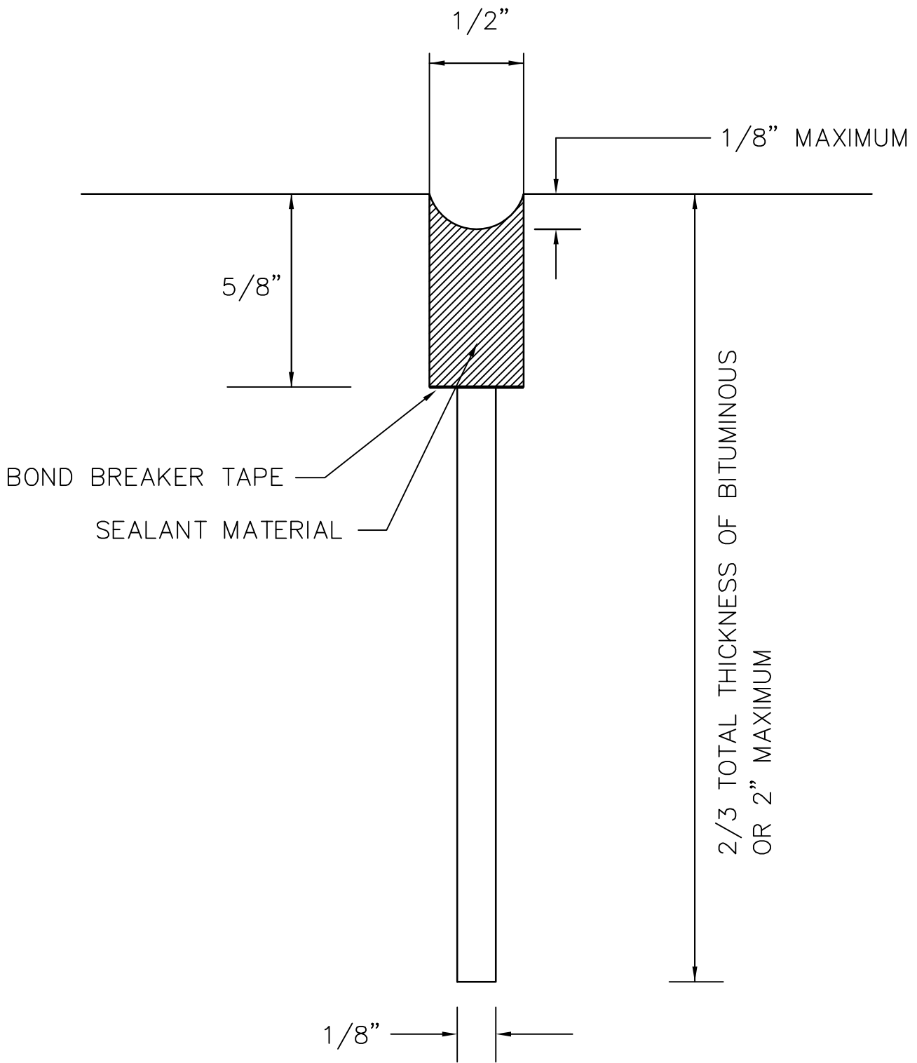
TYPICAL JOINT SECTION
